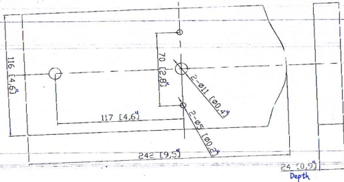
Line Drawing for Backplate of 30143.
