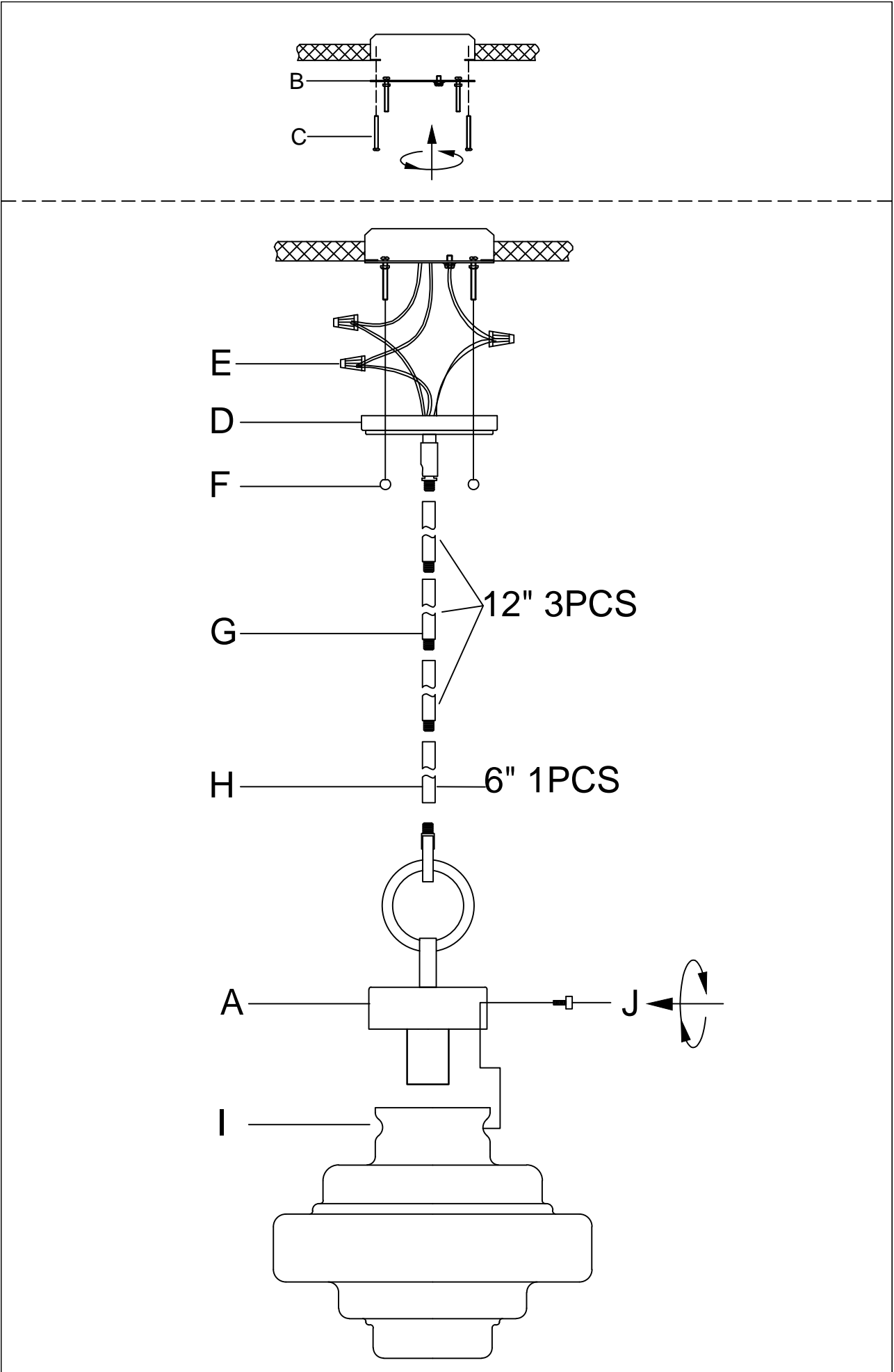
Run wire through stems and combine stem lengths to meet desired mounting height
