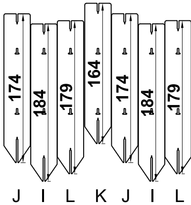
Part I front view
