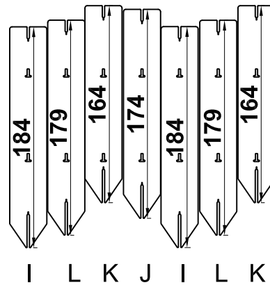
Part IV front view
