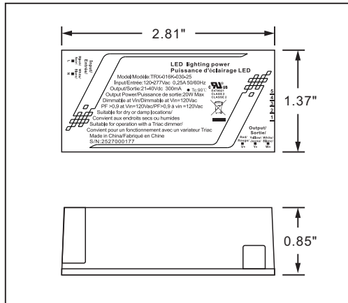
LED DRIVER DIAGRAM
