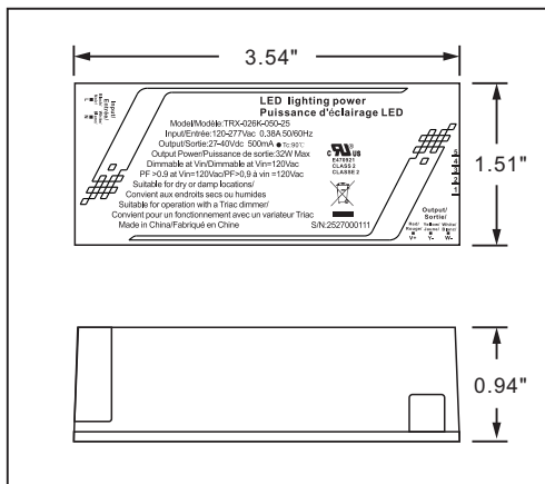
LED DRIVER DIAGRAM
