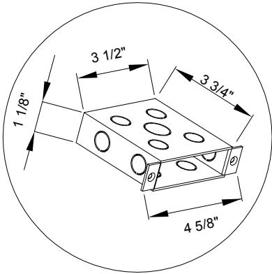
Slim Outlet Box Dimensions
