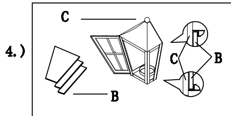
Step.4: Insert glass(B) and secure using glass clips
