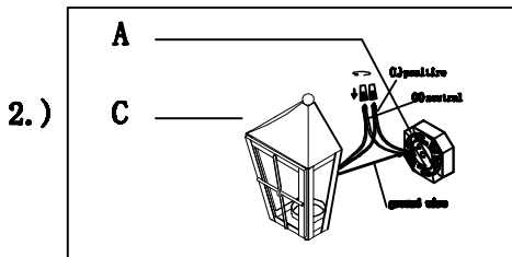
Step.2: Wire fixture to wires in outlet box. C copper wire is for Ground.
