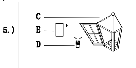
Step.5: Install GU24 bulb(D) and cover with Candle Cover(E)
