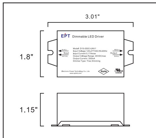
LED DRIVER DIAGRAM
